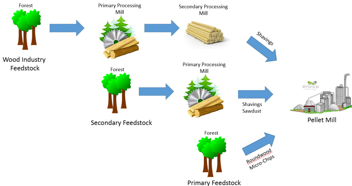
Figure 5. Typical Process Flow Chart
